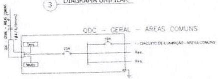
3 DIAGRAMA UNIFILAR
